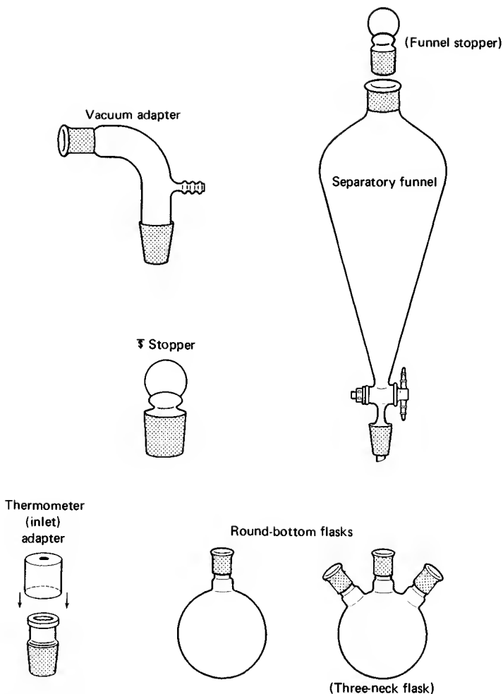
Fig. 19 Some jointware.
